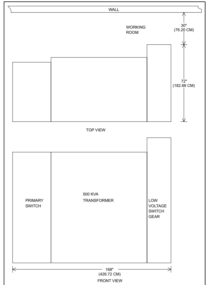
Figure 7. Conventional Secondary Unit Substation.
