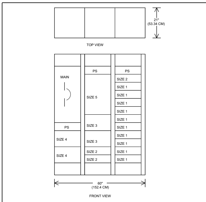
Figure 4. Advanced Design IT MCC (IT MCC).
