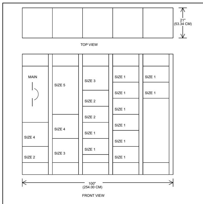
Figure 3. Conventional Motor Control Center (MCC).
