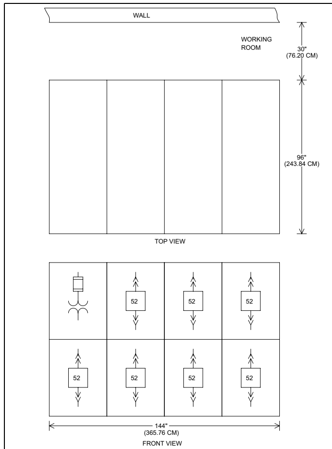
Figure 5. Standard Metal-Clad Switchgear.
