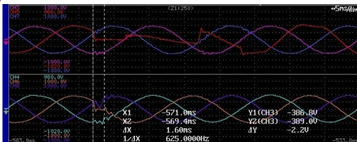
Figure B-1: Single-phase outage, output voltage recover in 1.6 ms, input voltage on top, output voltage below.
