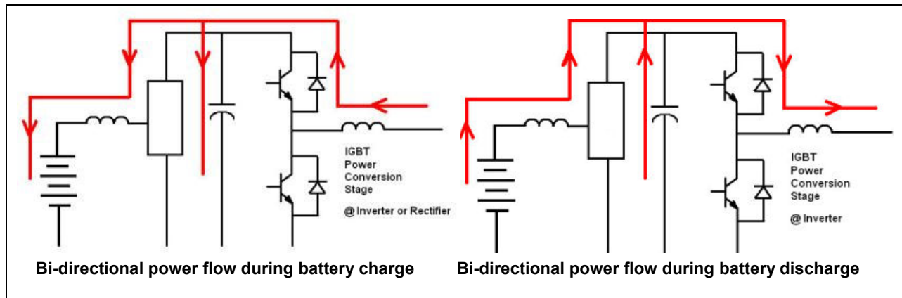
Figure 5: Bidirectional power flow diagrams
